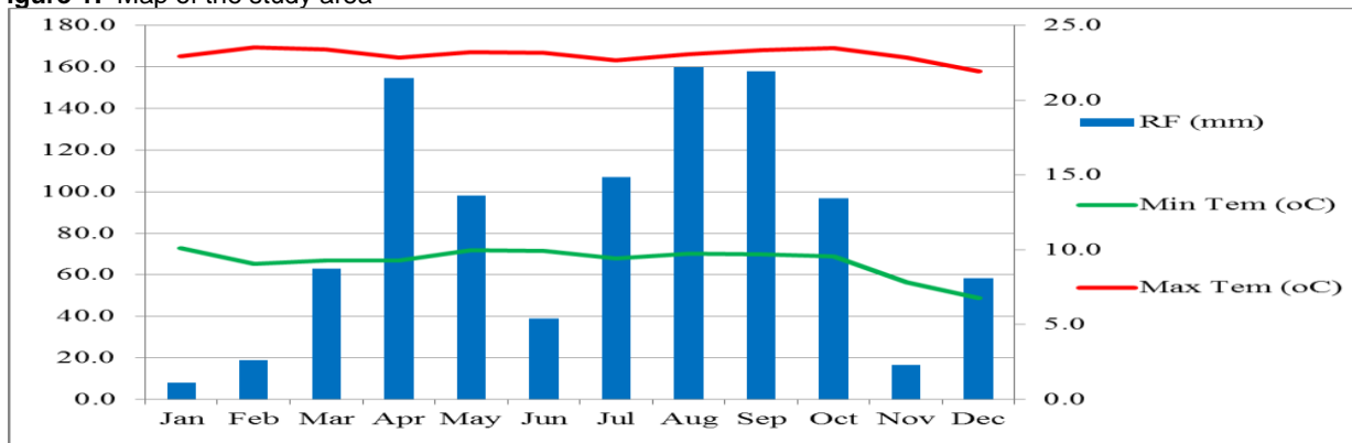
Figure 2: The Sinana district's average monthly rainfall (mm) and maximum and minimum temperatures (°C).
