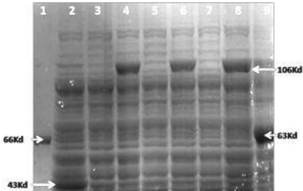
Figure 3. Protein profiles of E. coli BL21 expressing inulosucrase enzymes, resolved on 10% resolving gel by SDS-PAGE. Lane 1, BSA 66 kd; Lane 2, pMAL-p2 control; Lane 3, pMAL-p2 lacI Q ; Lane 4, pMAL-p2 lacI Q - inuJ 106kd; Lane 5, pMAL-p2 lacI Q ; Lane 6, pMAL-p2 lacI Q - inuJ 106kd; Lane 7, pMAL-p2 lacI Q ; Lane 8, pMAL-p2 lacI Q - inuJ 106kd; Lane 9, pET- inuJ 63kd.
