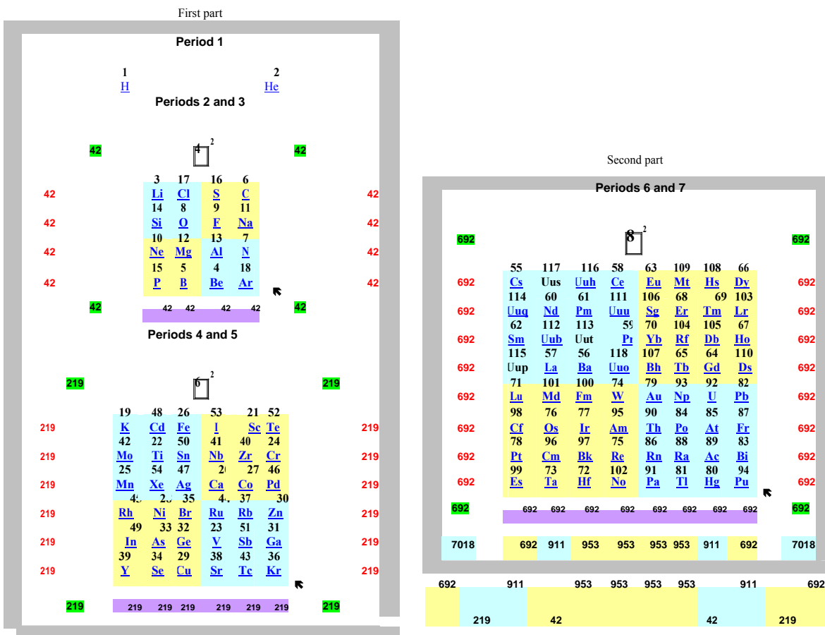
Figure 10. Mathematical position of chemical elements in digital tables of elements.
