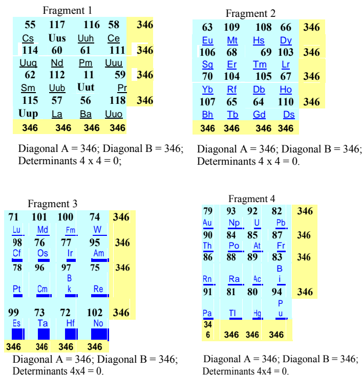
Figure 11. chemical elements from the sixth and seventh period interconnected through the code 346
