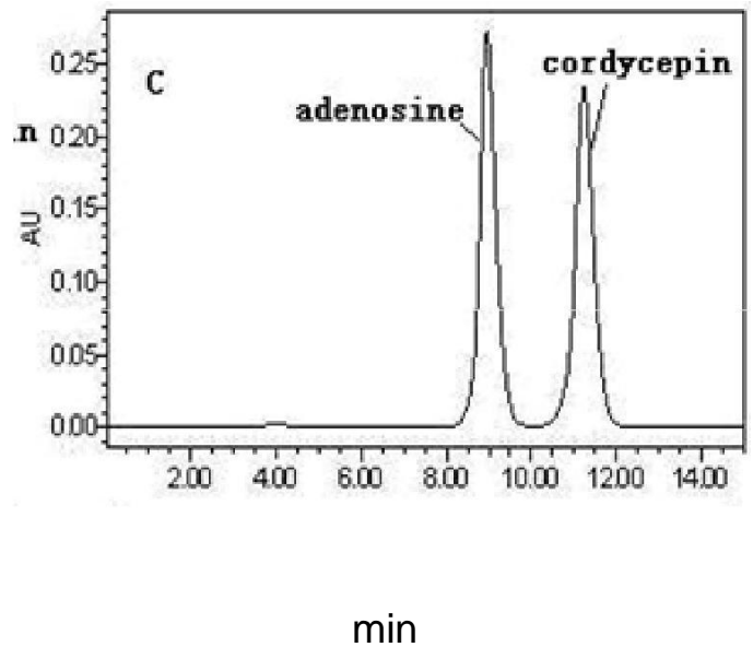
Figure 1c. Retention time of adenosine and cordycepin under different percentage of water and methanol in mobile phase; Water-methanol (92:8, V/V) Retention time of adenosine and cordycepin 8.955 and 11.230 min, respectively.
