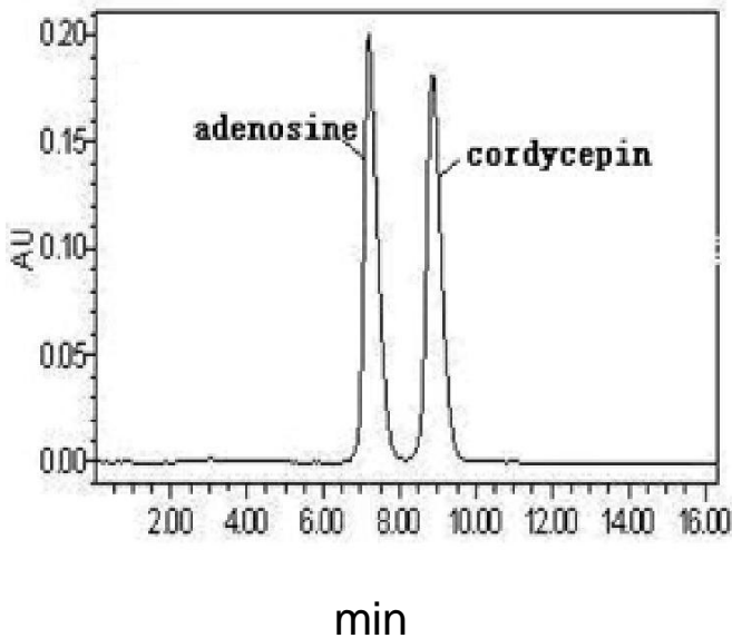
Figure 1b. Retention time of adenosine and cordycepin under different percentage of water and methanol in mobile phase; water-methanol (90:10, V/V), retention time of adenosine and cordycepin 7.204 and 8.864 min, respectively.
