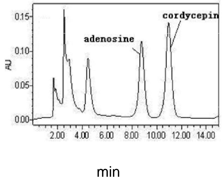
Figure 1d. Retention time of adenosine and cordycepin under different percentage of water and methanol in mobile phase; A C. militaris sample separated under mobile phase consisting of water-methanol (92:8, V/V).
