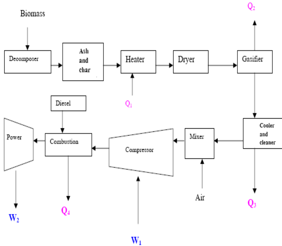
Figure 7. Advanced biomass power with diesel engine (Omer, 2006).
