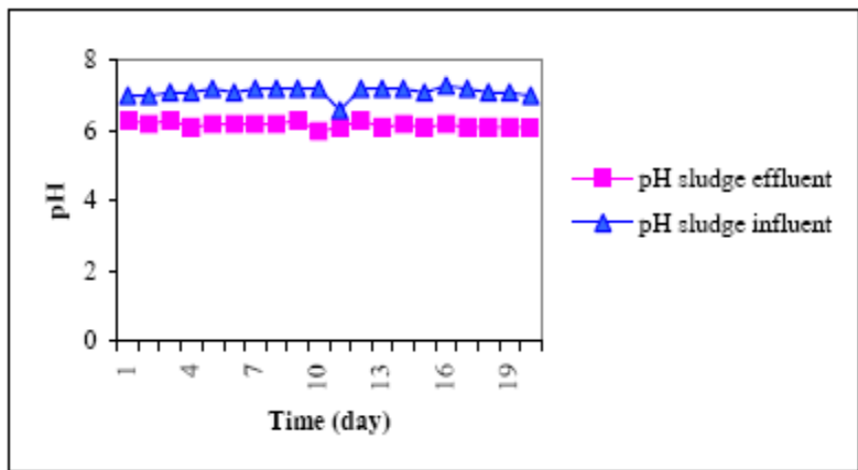
Figure 6. Potential of hydrogen (pH) sludge before and after treatment in the digester (Omer, 2006).
